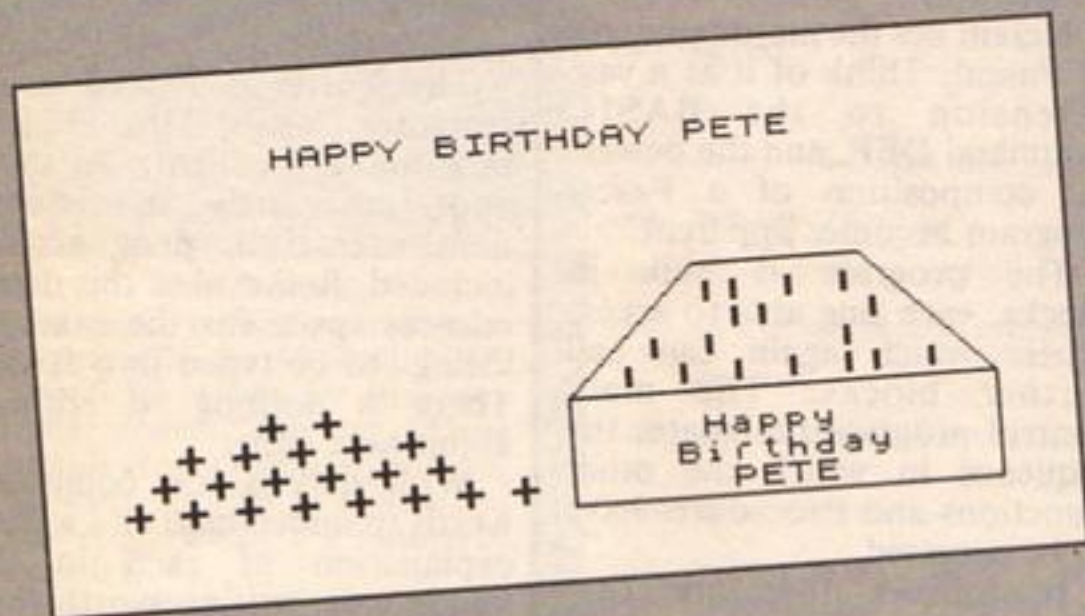
Listing 2
